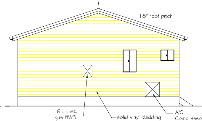
ELEVATION D
